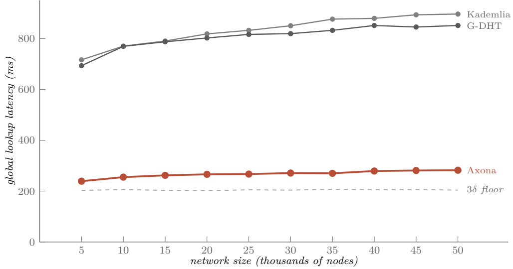
Figure 4: Global lookup latency versus network size at every 5,000 from 5,000 to 50,000 nodes (10× scaling), plotted against the Dabek 3\delta analytical floor (gray dashed). Kademlia climbs from 716 to 896 ms as the log- N hop tax compounds; G-DHT tracks Kademlia almost identically on global lookups (the geographic prefix only helps regional cells). Axona hugs the floor in a tight 239–282 ms band across the whole range ( 1.17\text{--}1.38\times the 3\delta floor) and is essentially flat from 15,000 nodes onward — adding 35,000 more nodes raises latency by 20 ms total. All success rates 100%. Data: sim v0.93.0 / @axona/protocol v1.1.3, May 2026.
