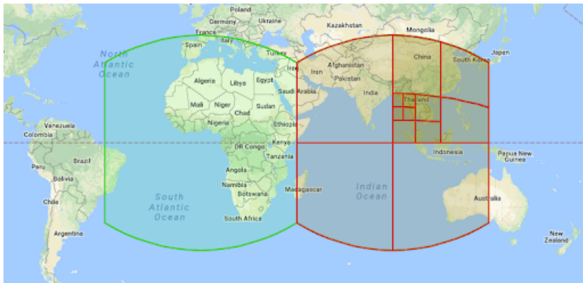
Figure 1: S2 cell decomposition of Earth’s surface, projected through six cube faces along a Hilbert space-filling curve. Nearby points on the globe land at numerically close cell IDs; XOR distance in identifier space therefore approximates physical distance, for free. G-DHT uses the top 8 bits of each node ID to encode the S2 cell of the node’s claimed position.
